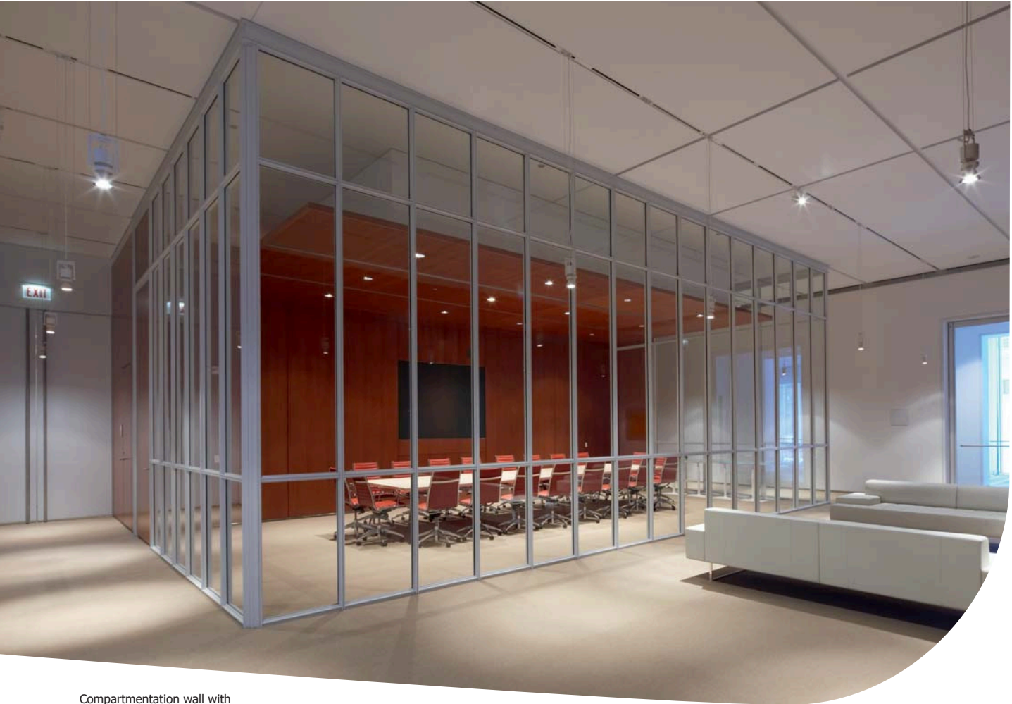
Compartmentation wall with Pilkington Pyrostop ® – Chicago Art Institute, Chicago (USA).
